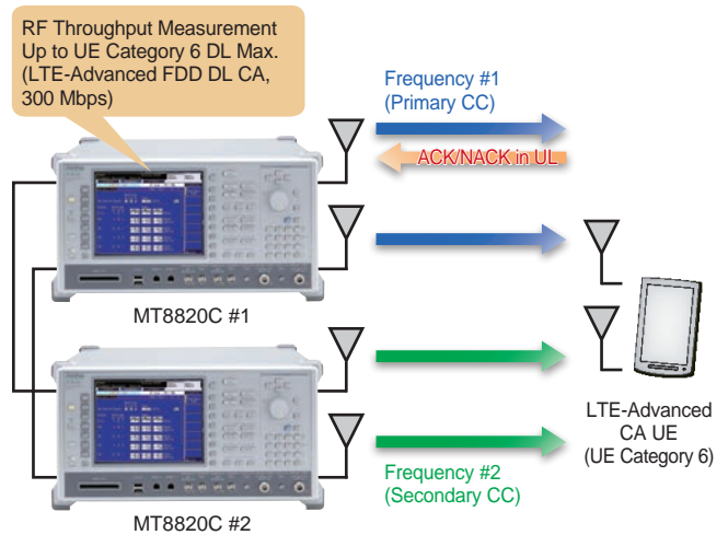
Sample MT8820C connection
